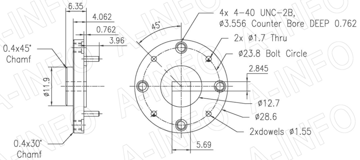
FUGP400 (equivalent to UG-383/U)
